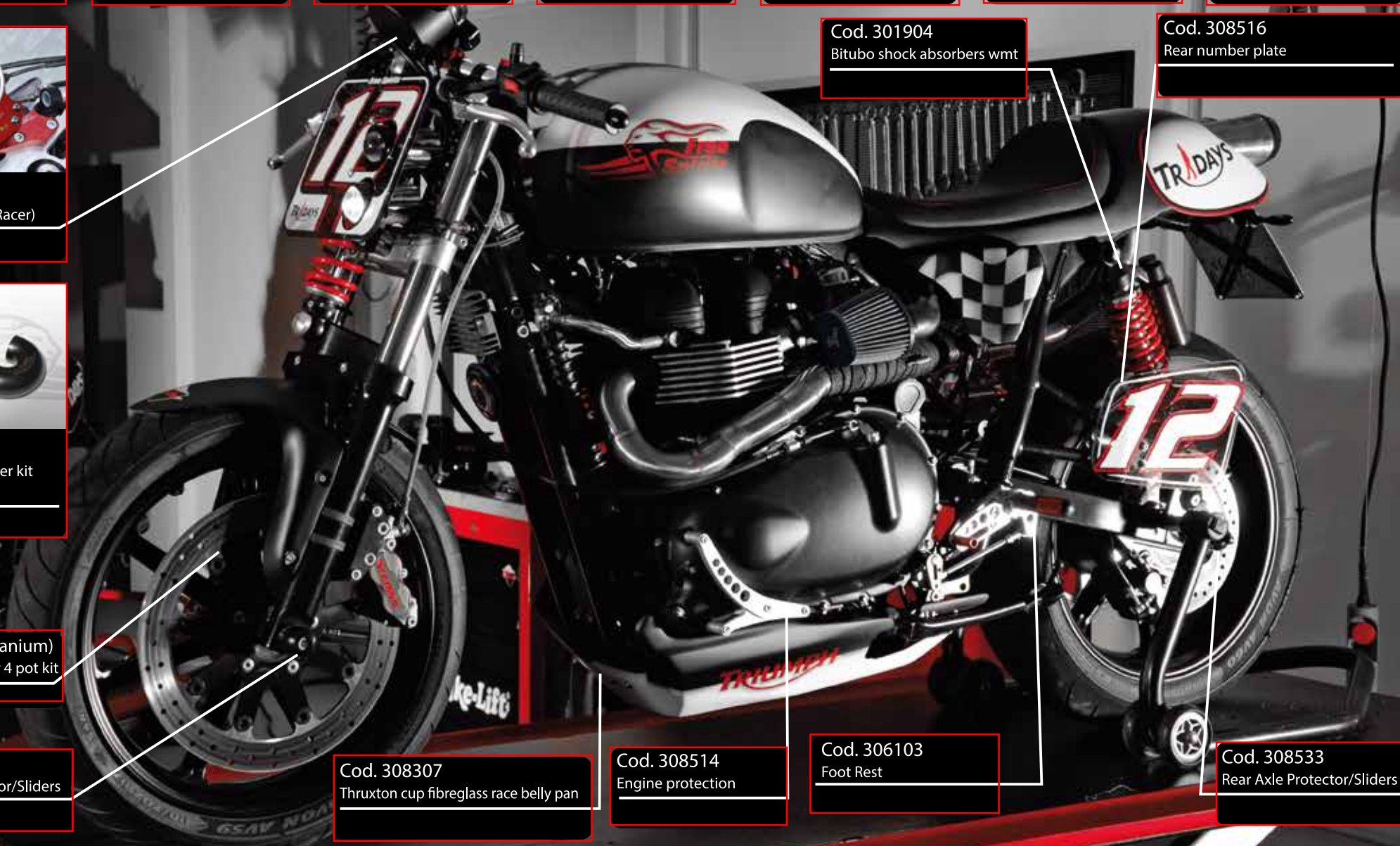
Cod. 302302 "Cafè racer" Triple Clamps
